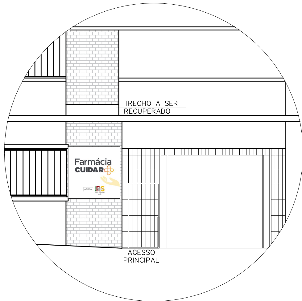
DET.01 - FACHADA PRINCIPAL ESC: 1/75
